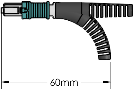
FORMABLE BOOT @ 90°
